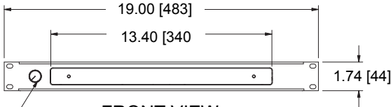
FRONT VIEW (LT-1RA)
