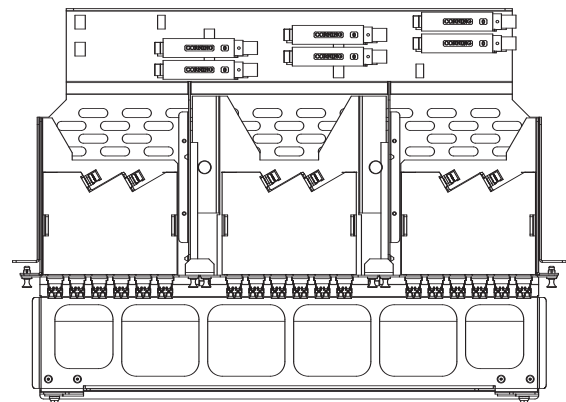
Pretium 3-Module Housing (PCH-M3-01U), Top View | Drawing ZA-2979
