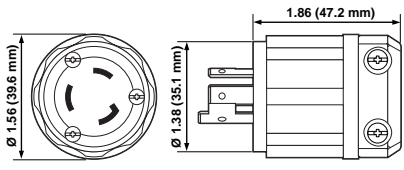
LOCKING PLUG Cat No. 23CM-11C
