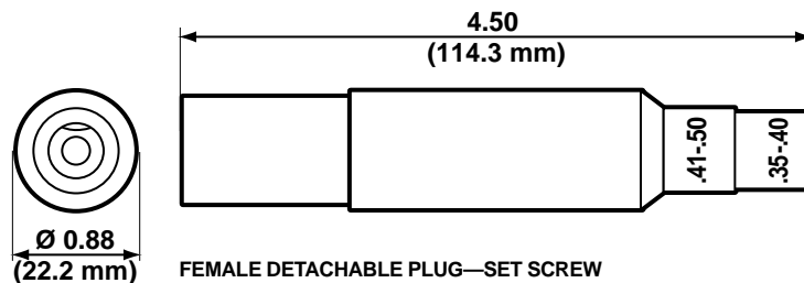
FEMALE DETACHABLE PLUG—SET SCREW Cat. No. 15D22
