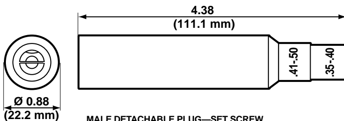
MALE DETACHABLE PLUG—SET SCREW Cat. No. 15D21
