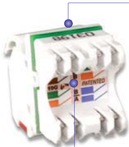
T568A and T568B wiring compatible
