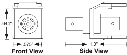
ST QuickPort® Adapter
