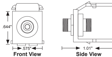
FC QuickPort Adapter
