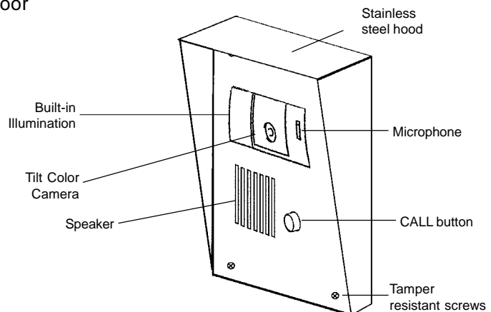
KB-DAR or KC-DAR Video Door Station in KA-FSH Housing
