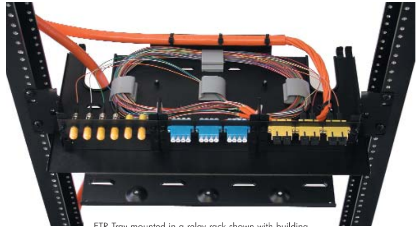
FTR Tray mounted in a relay rack shown with building cable routed to adapter panels.
