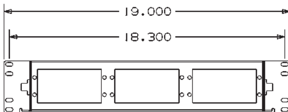
FTR front view with cutouts for FSP Adapter Panels
