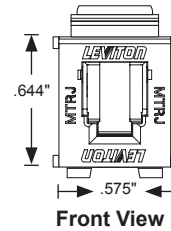
MT-RJ QuickPort Adapter
