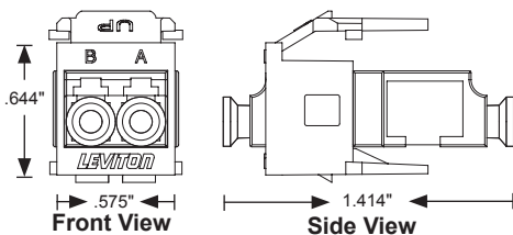
LC QuickPort Adapter
