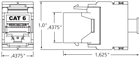
CAT 6A Shielded Jack - Front View, Side View
