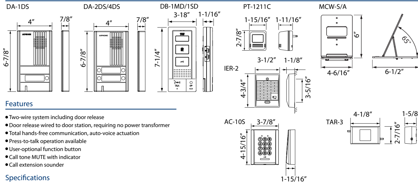
AC-10S Vandal resistant access control keypad, surface mount
