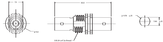
Threaded ST Compatible Connector Adapter | Drawing CPC-220-3-5
