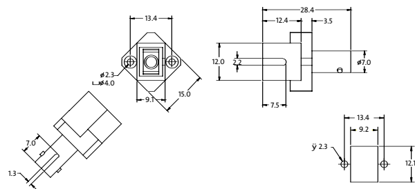
ADP-STSC-MCXSF-NLS | Drawing ZA-2212
