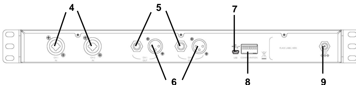
Rear View
