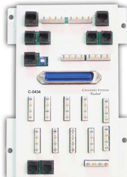
C-0434 KSU Interface Module
