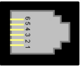
RJ11 jack Front Face
