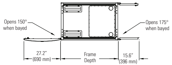
Top View (Server Top Panel with Vertical Exhaust Duct knockout)
