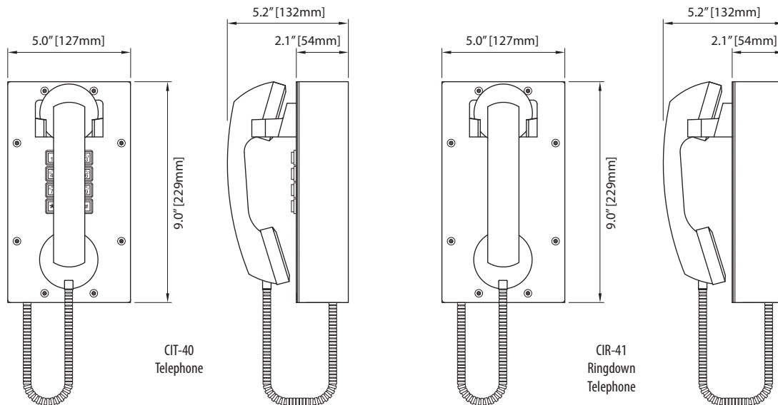
CIT-40 & CIR-41 Ringdown – Correctional Institute Telephones
