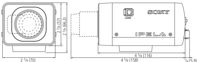
Unit: inches (mm)
