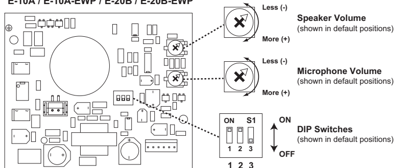
Rear View of the Speaker Phone models: E-10A / E-10A-EWP / E-20B / E-20B-EWP
