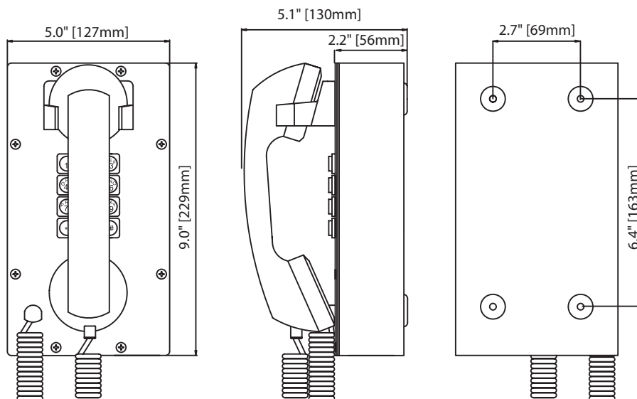
SCT-10/20/30/40 Steel Compact Telephones
