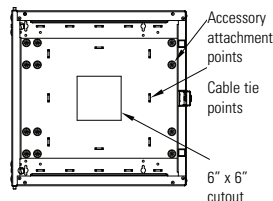
Rear Panel View (Interior Detail)
