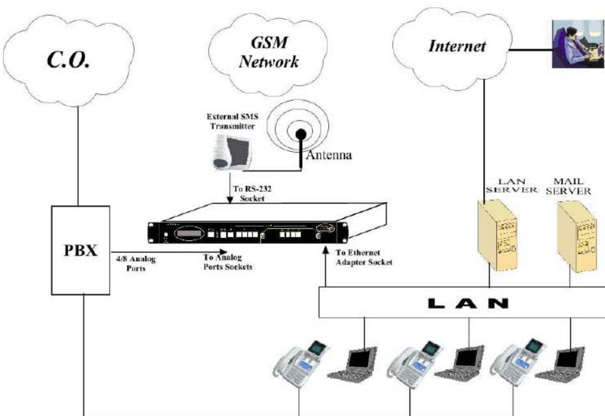
Figure 1-1: Voice Mail System connections
