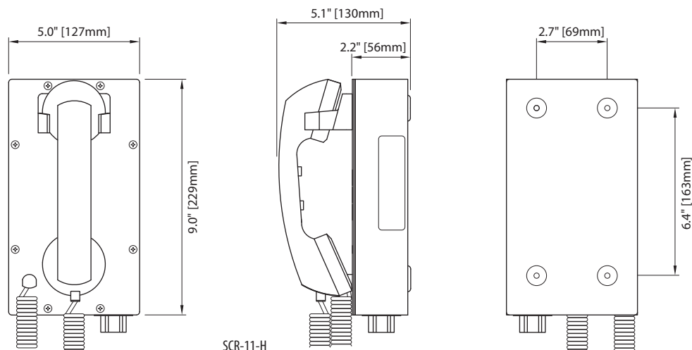
SCR-11-H / SCR-41-H Steel Compact Ringdown Telephones
