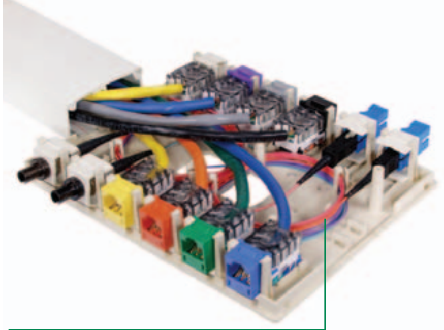
Integrated fiber storage posts facilitate the storage of 1m of fiber cable (4, 6, 12-port).
