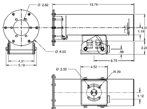
OUTLINE DRAWING
