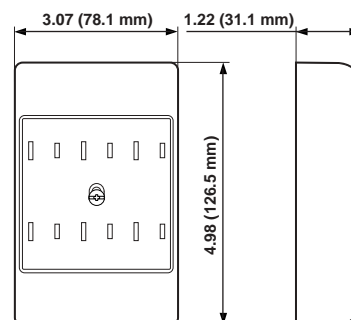
DUPLEX-TO-SIX OUTLET ADAPTER Cat. No. 49687
