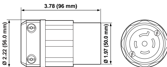
LOCKING CONNECTOR Cat. No. 2523
