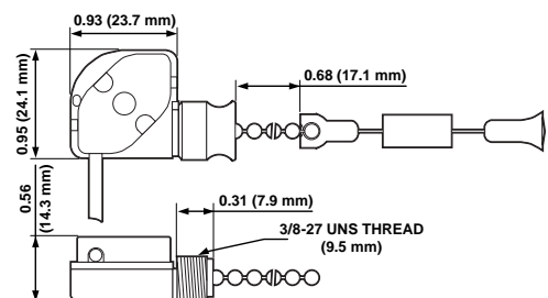
COMPACT PULL CHAIN SWITCH Cat. No. 10097-8
