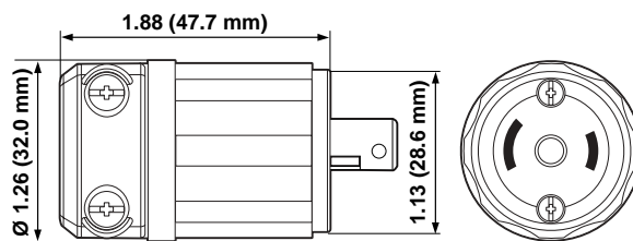
MIDGET LOCKING PLUG Cat. No. ML2-P
