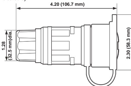
WETGUARD™ 15A LOCKING CONNECTOR
