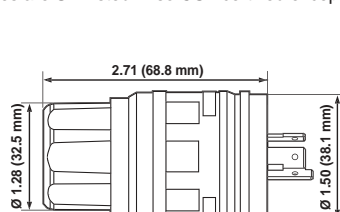
WETGUARD™ 15A LOCKING PLUG
