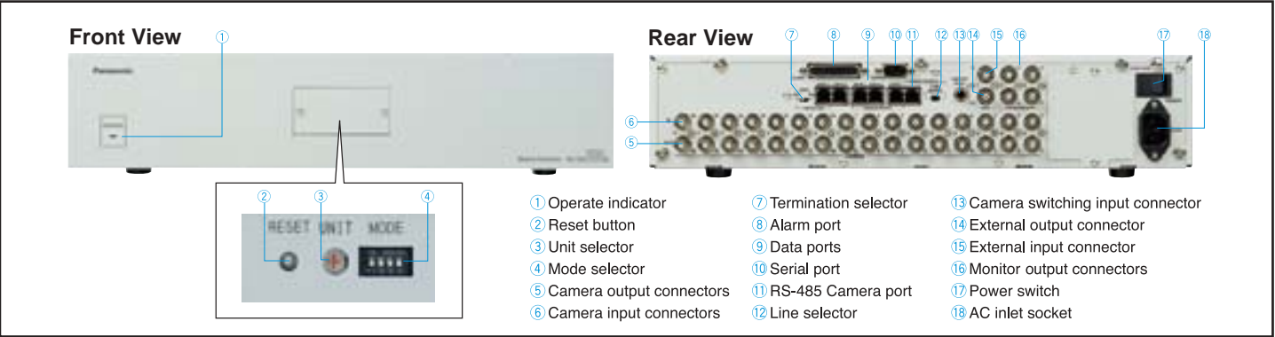
System Controller; WV-CU360C
