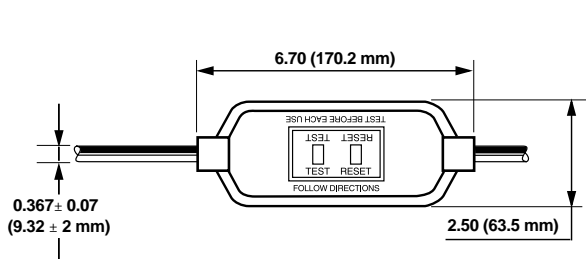
15A AUTO GFCI CORD Cat. No. 66591-2C
