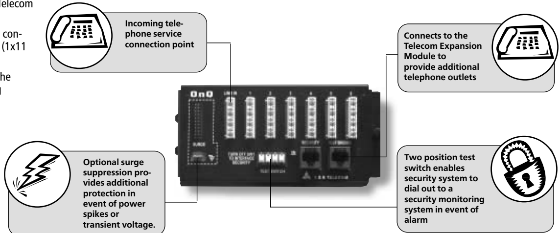
1x6 Basic Telecom Module
