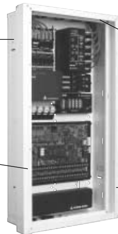
28" PLUS Series Enclosure
