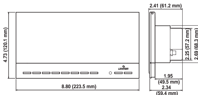
TOSCANA CONTROLLER—Cat. No. HCCPG-1TW
