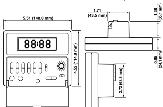
BASIC WALL MOUNTED PROGRAMMER—Cat. No. 6312
