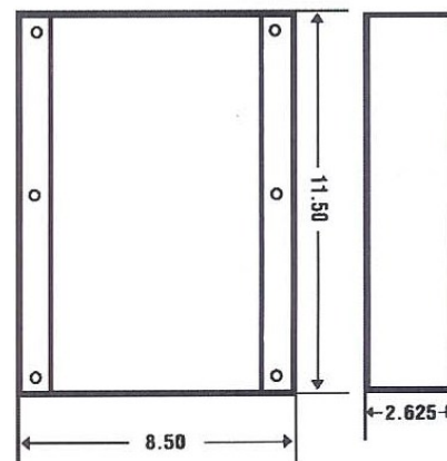
MOUNTING BOX
