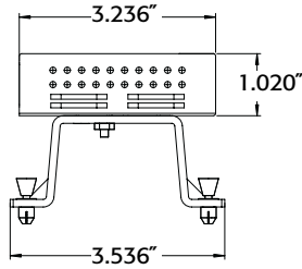
Side Panel
