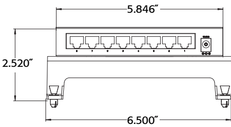
Back Panel
