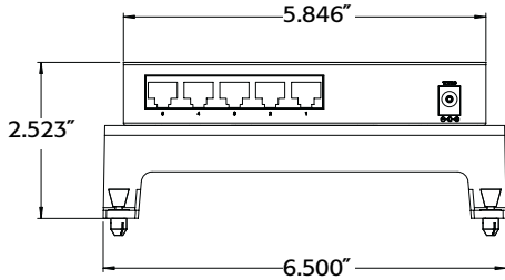
Back Panel
