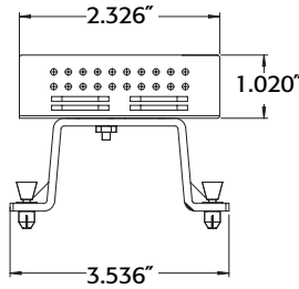
Side Panel
