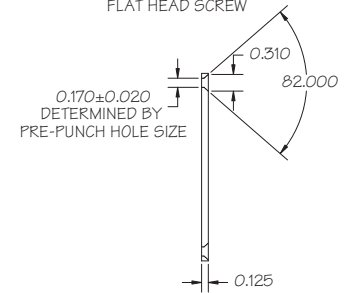
COUNTERSINK FOR 6-32 FLAT HEAD SCREW
